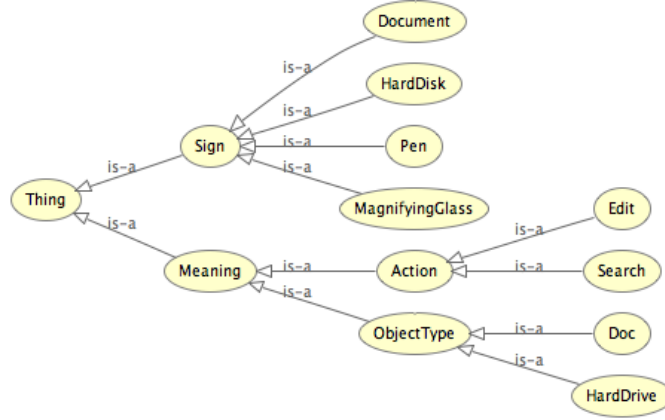
Figure 2: The ComputerIcon ontology, showing the concept names and their relation.
