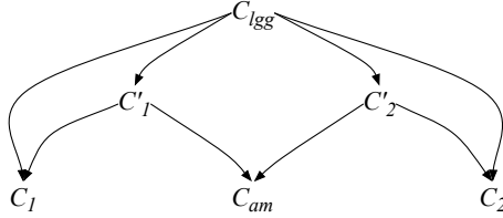
Figure 1: A diagram of amalgamation from descriptions C_1 and C_2 with an amalgam C_{am} . Arrows indicate the subsumption of the target by the source of the arrow.
