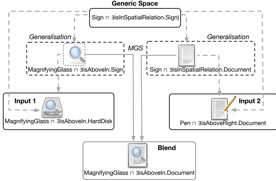
Figure 3: Blending the SearchHardDisk and EditDocument icon concepts into a new concept representing a search-in-document icon. Sign’s meanings are not represented.
